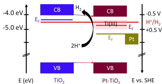
Scheme 1. Electronic Band Positions of Ti(III) in Pt–TiO 2 Based Nanocomposite
