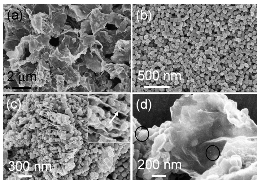
Figure 1. FESEM images of (a) GO, (b) cuboid shaped \text{TiO}_2 NCs, (c) \text{TiO}_2 -N-hrGO, and (d) Pt- \text{TiO}_2 -N-rGO nanocomposites. Inset of (c) shows magnified FESEM image of the corresponding sample showing \text{TiO}_2 NCs in between the N-hrGO sheets.
