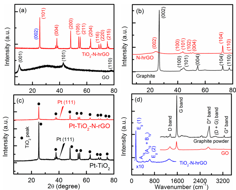
Figure 3. XRD patterns of (a) GO and TiO 2 -N-hrGO, (b) graphite and N-hrGO, and (c) Pt-TiO 2 and Pt-TiO 2 -N-rGO. (d) Raman spectra of graphite powder, GO, and TiO 2 -N-hrGO nanocomposite.
