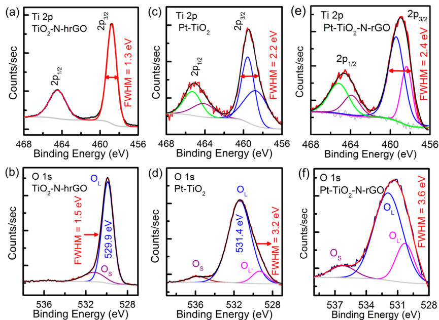
Figure 4. (a, c, e) Ti 2p and (b, d, f) O 1s region XPS spectra of (a, b) TiO 2 -N-hrGO, (c, d) Pt-TiO 2 , and (e, f) Pt-TiO 2 -N-rGO nanocomposites.
