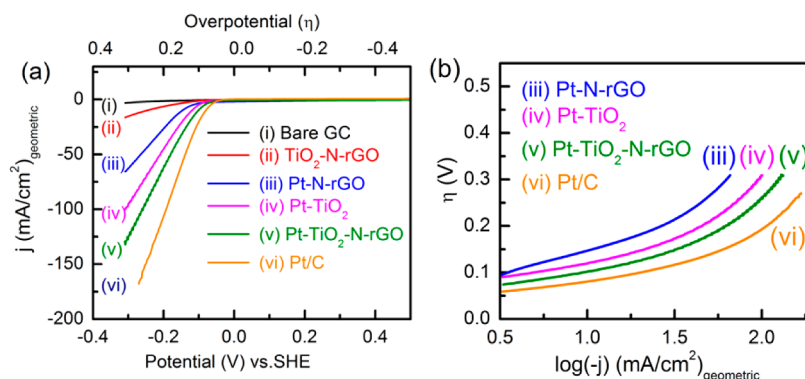
Figure 5. (a) HER activity of the different nanocomposite catalysts in 0.1 N H 2 SO 4 at a scan rate of 100 mV·s -1 . (b) Tafel plot of the different Pt-based nanocomposites. The current density was measured considering the geometric area of the working disc GC electrode.
