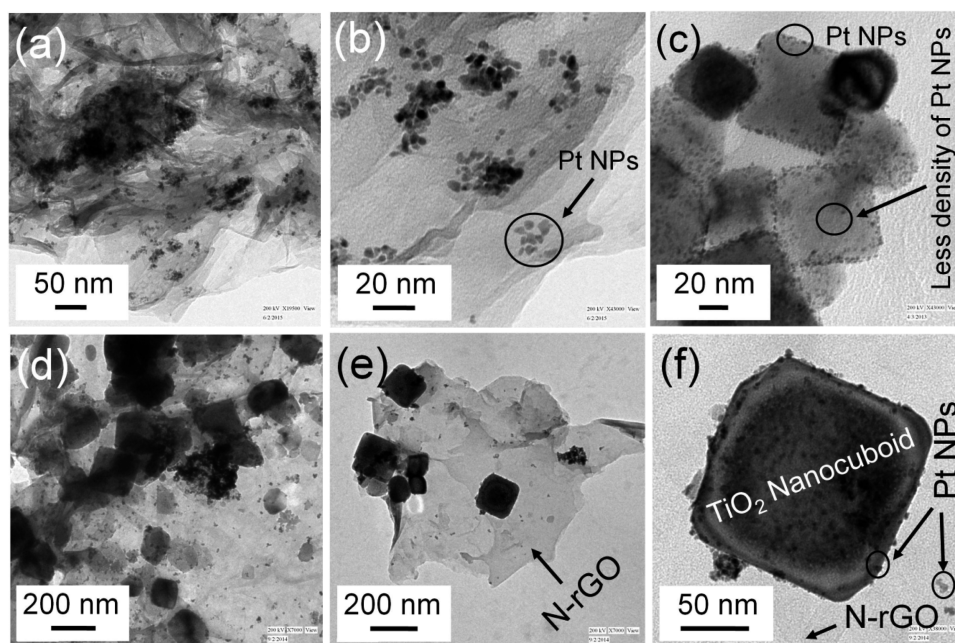
Figure 2. (a, b) TEM images of Pt-N-rGO nanocomposite depicting the sheet structures of N-rGO decorated with chemically reduced Pt NPs. (c) TEM image of Pt- \text{TiO}_2 NCs showing the selective photodeposition of <5 nm Pt NPs majorly at the edges of the cuboid shaped \text{TiO}_2 NCs. (d, e, f) Ternary nanocomposite of Pt- \text{TiO}_2 -N-rGO shows the \text{TiO}_2 NCs in between the N-rGO sheets and deposition of Pt NPs on both \text{TiO}_2 NCs and N-rGO sheets.
