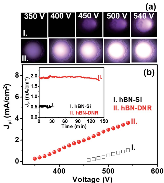
Fig. 6 (a) The microplasma illumination images and (b) plasma current density versus applied voltage characteristics with the inset showing the plasma illumination stability, the life-time, of the microplasma devices, which were fabricated using I. hBN-Si and II. hBN-DNR as cathode materials.
