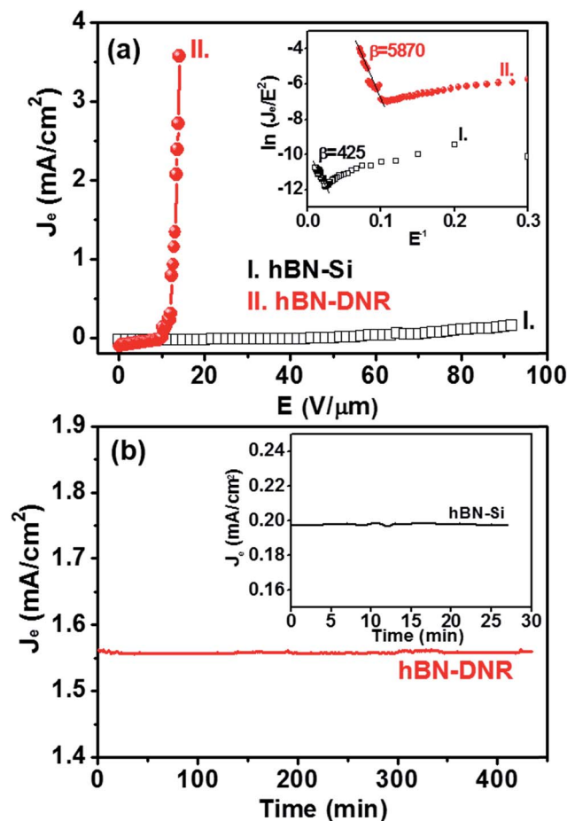
Fig. 5 (a) The field electron emission properties ( J_e - E curves) with F-N plots as inset for I. hBN-Si and II. hBN-DNR and (b) the current density versus time curves of hBN-DNR. The inset in (b) shows the current density versus time curve of hBN-Si.
