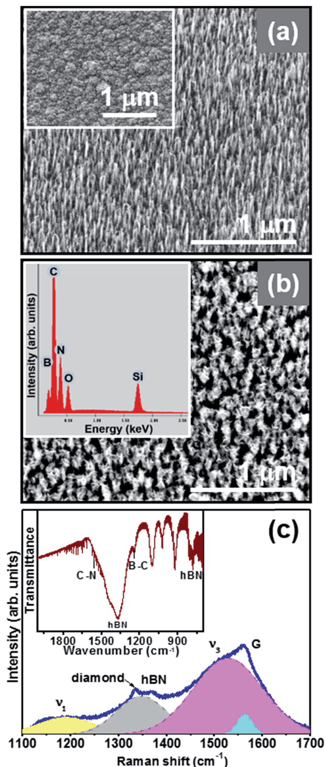
Fig. 2 (a) Tilted view SEM image of bare DNRs (inset shows the SEM morphology of NCD film). (b) Tilted view SEM image for hBN-DNR with EDX spectrum shown as inset. (c) Micro-Raman spectrum of hBN-DNR with FTIR spectrum shown as inset.
