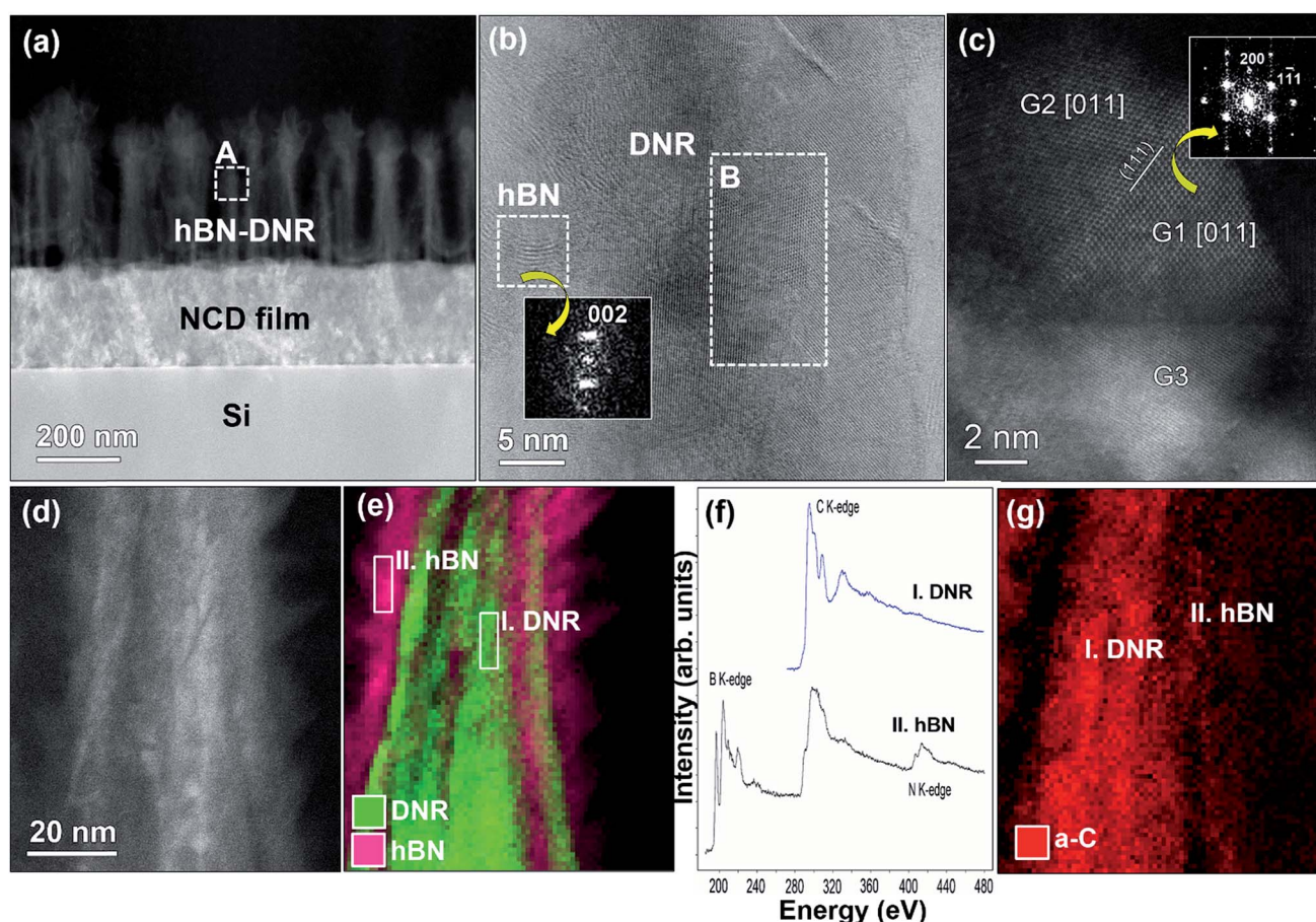
Fig. 4 (a) Typical cross-sectional HAADF-STEM image of the hBN-DNR. (b) HR-STEM image of a single hBN-DNR corresponding to region “A” of (a), with the FT patterns displayed in the inset of (b), disclosing the hBN phase. (c) Higher magnification HR-STEM image corresponding to the region “B” of (b), revealing the diamond structure and the FT pattern shown as in the inset of (c) evidences the crystalline nature of the diamond. (d) Typical HAADF-STEM micrograph of the hBN-DNR together with (e) composed EELS elemental mapping for hBN (pink) and DNR (green). (f) Summed EELS core-loss spectra taken from the diamond and hBN regions in the maps in (e). (g) EELS mapping of (d) disclosing the presence of a-C in hBN-DNR heterostructures.
