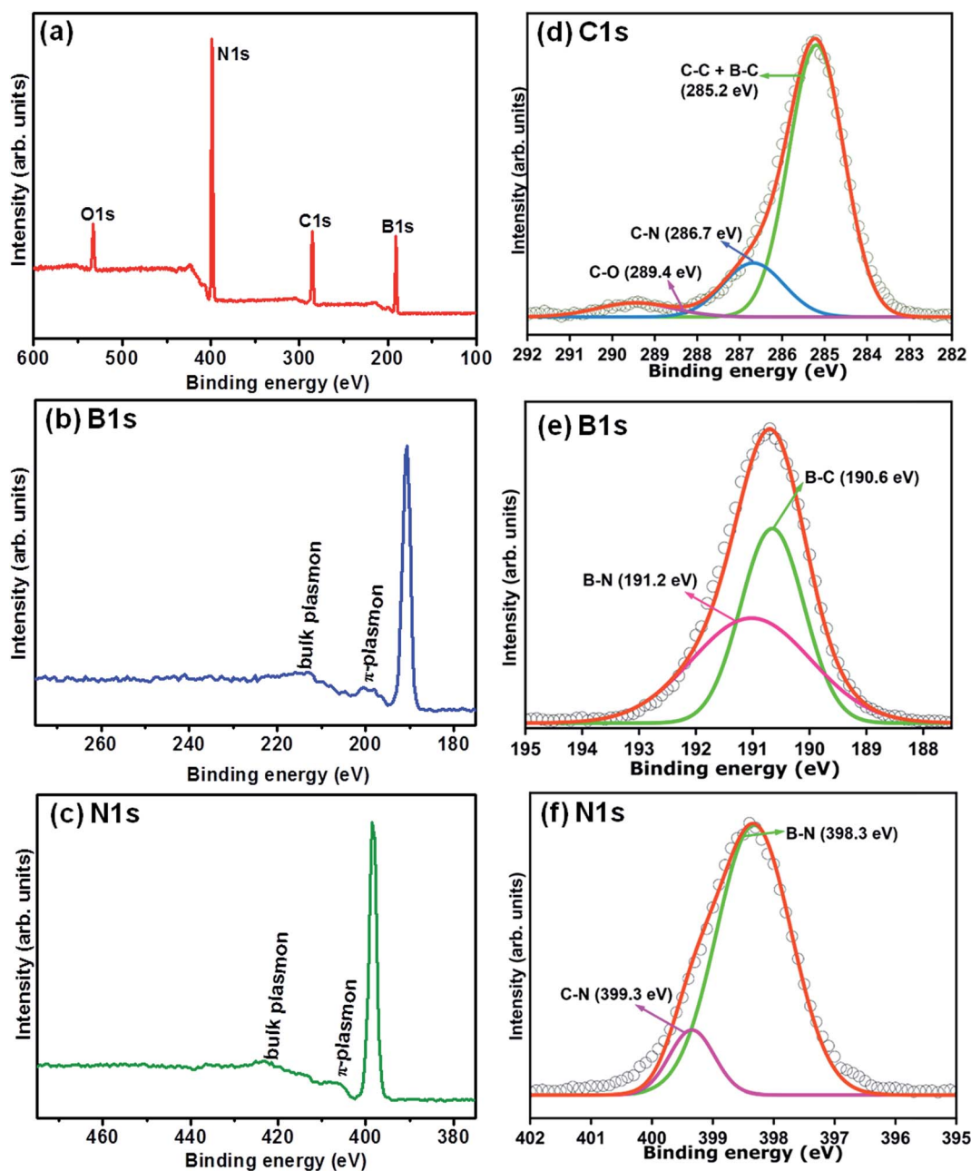
Fig. 3 (a) XPS survey spectrum of hBN-DNR, (b) the B1s and (c) the N1s peaks at a higher magnification, (d)–(f) deconvolutions of C1s, B1s and N1s edges of hBN-DNR heterostructures, respectively.
