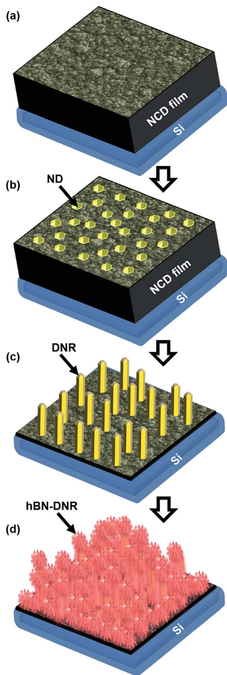
Fig. 1 Schematics of the fabrication process of hBN-DNR heterostructures: (a) growth of NCD film on Si substrates; (b) masking ND particles on NCD films; (c) reactive ion etching for forming DNRs and (d) growth of hBN nanowalls on DNRs.
