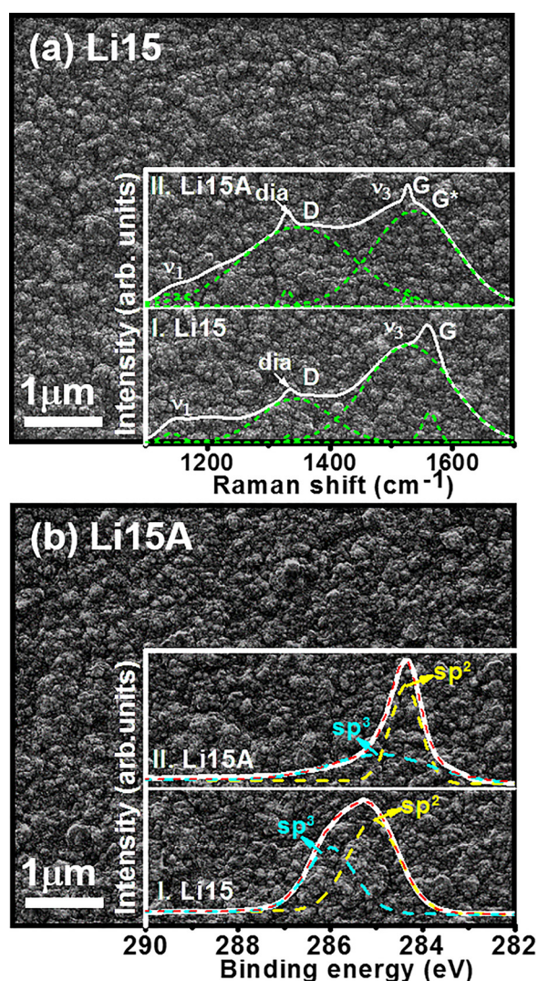
FIG. 2. SEM images of (a) Li15 films and (b) Li15A films; the inset in “a” shows the micro-Raman ( \lambda = 488.0 \text{ nm} ) spectra of I. Li15 and II. Li15A films; the inset in “b” shows the C1s XPS spectra of I. Li15 and II. Li15A films.
