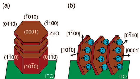
Figure 9. Schematic diagrams of (a) 1D and (b) 2D growth of ZnO nanostructures on ITO-glass. Nanospikes and nanopillars grow on the preferred plane (0001) forming the 1D nanostructures (a). In the case of nanowalls and nanodisks, \text{Cl}^- ions cap the (0001) facet of ZnO and thereby redirect growth on the (10 \bar{1} 0) plane, forming the 2D nanostructures (b).
